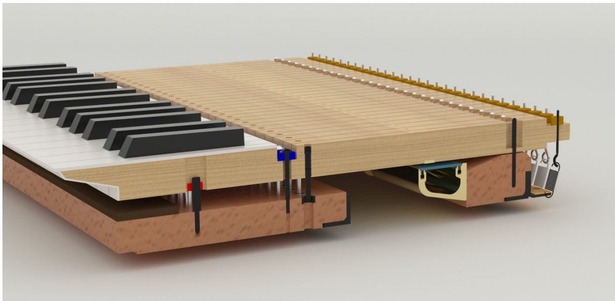
One-armed keyboard with pluck simulation and mounted Espressivo sensor rail on the front of the balance rail.
