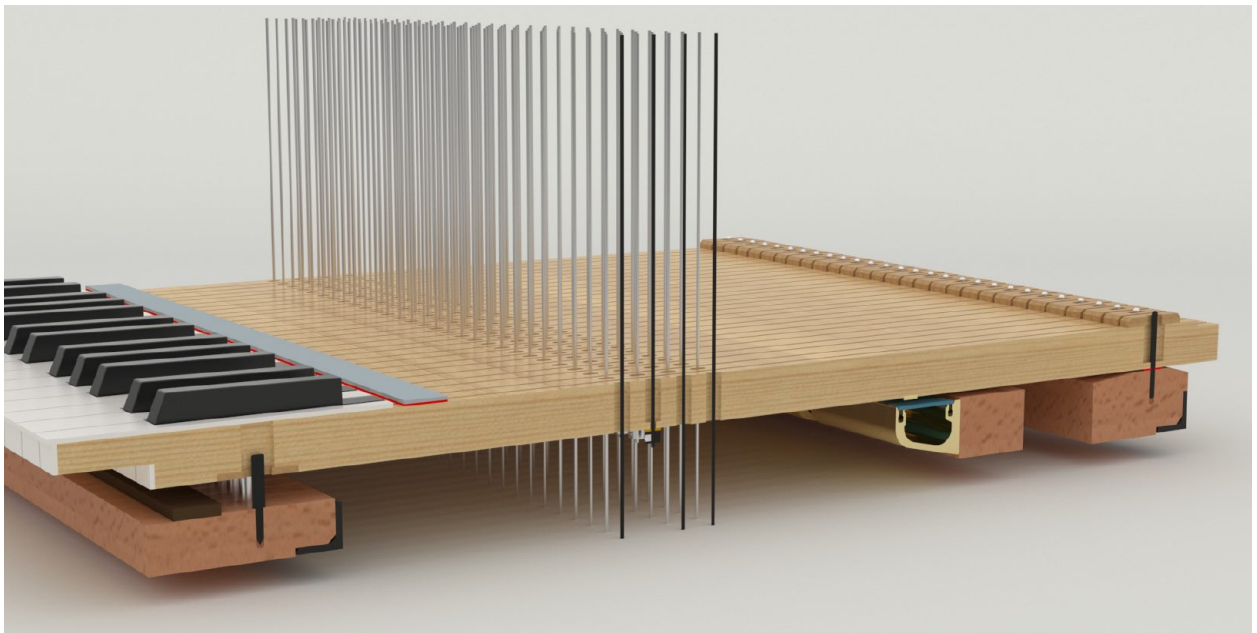
Keyboard for suspended mechanical action, with Espresso sensor bar on an additional support bar in front of the balance rail.
