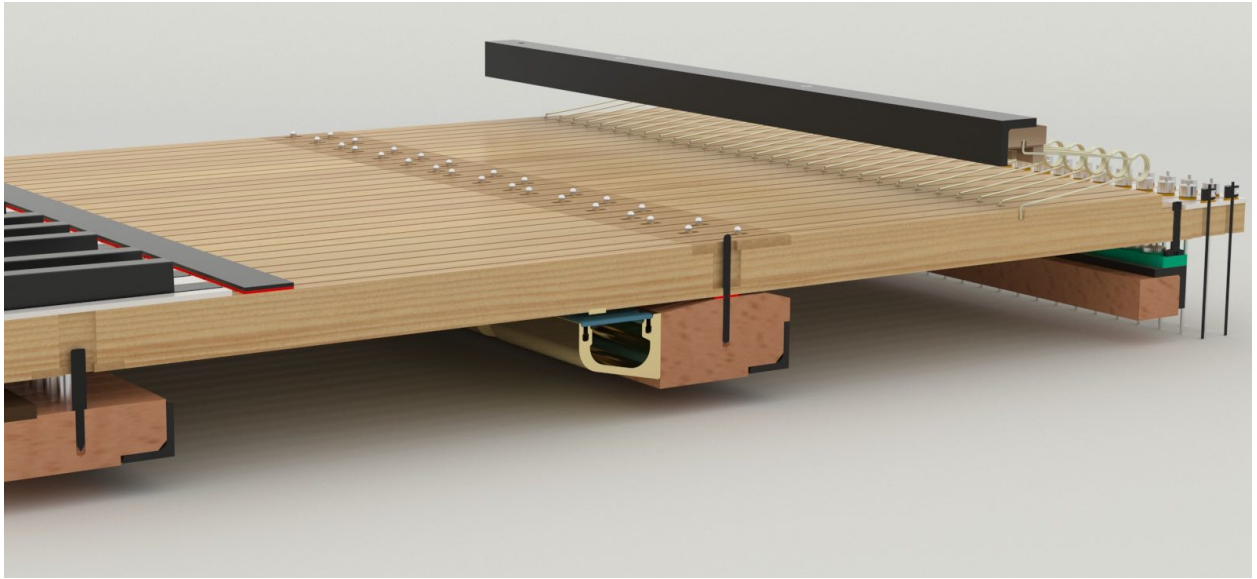
Two-armed keyboard with stop rail and Espresso sensor rail mounted on the balance rail.
