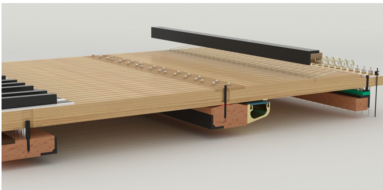
Two-armed keyboard with stop rail and Espressivo sensor rail in inverted mounting on the balance rail.
